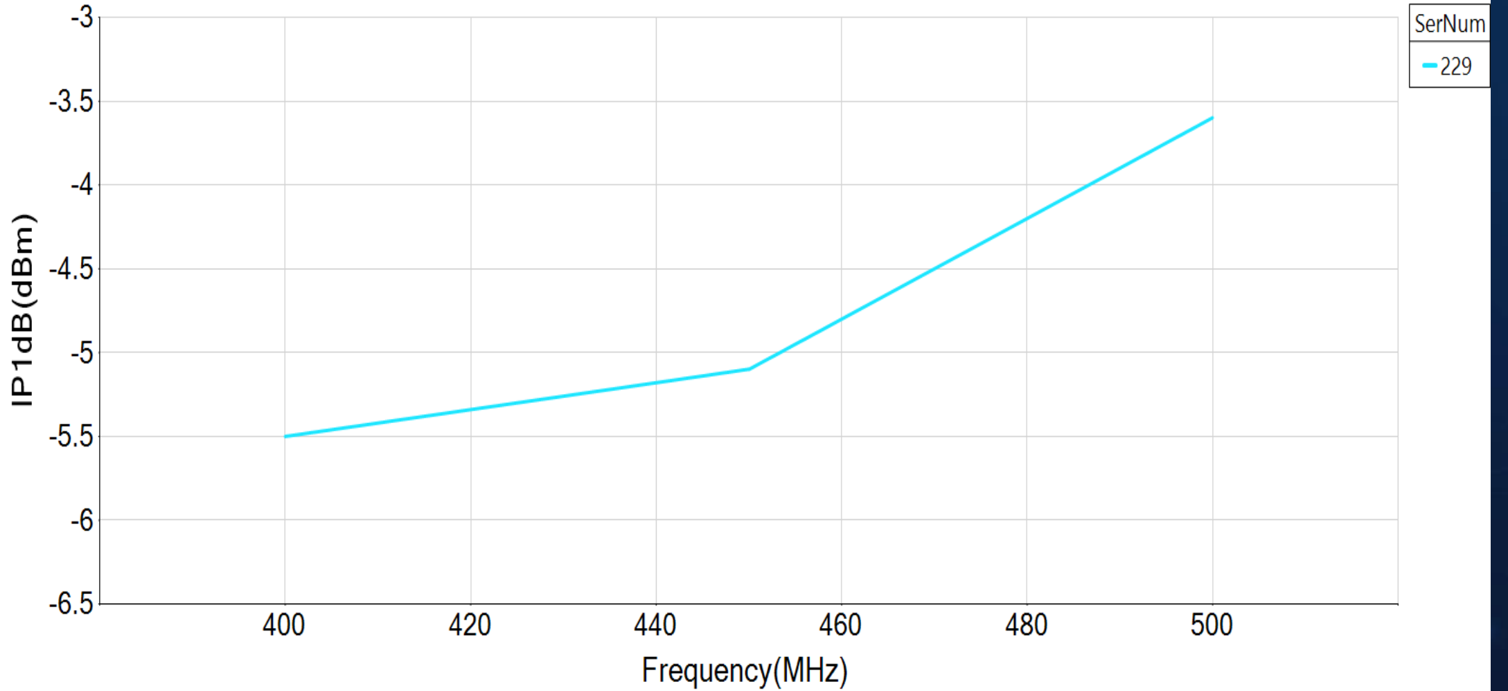
GRF5504 IP1dB vs Frequency
