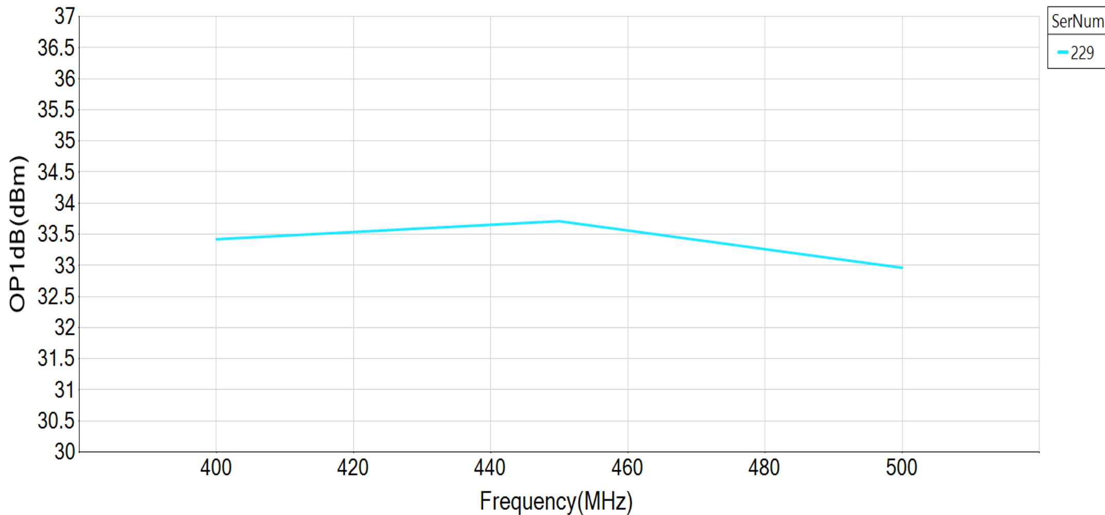
GRF5504 OP1dB vs Frequency
