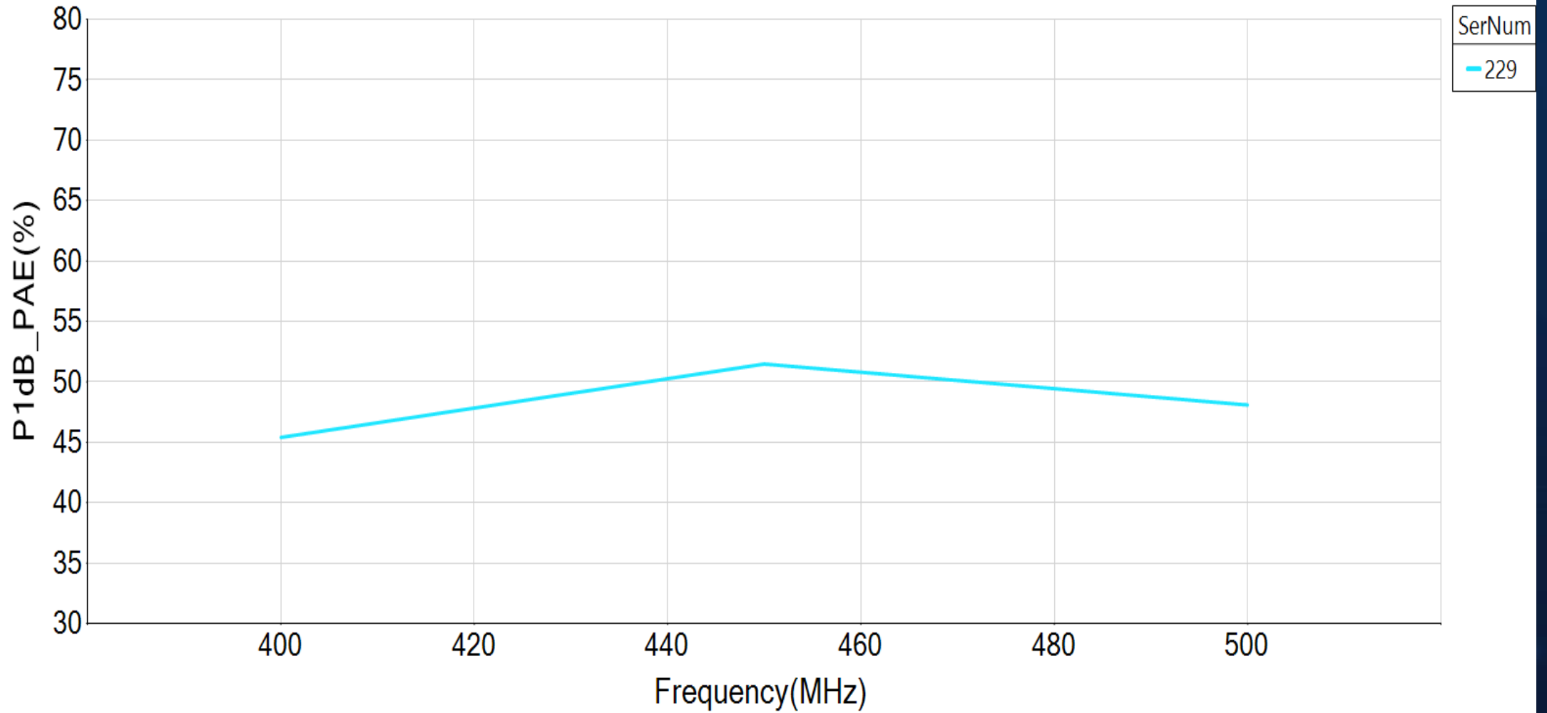
GRF5504 P1dB_PAE(%) vs Frequency
